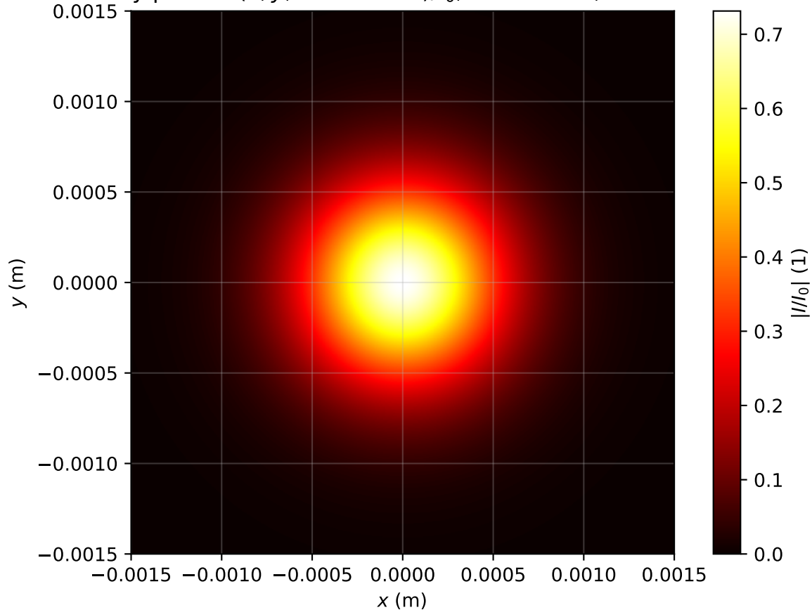
Intensity profile I(x, y, z = 1.990m)/I_0 , \text{Pin}=0.4\text{Pcr} , artificial time
